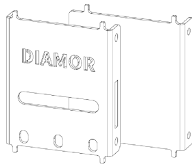
PART B ACCS-GATE-0440 ChainLink Double Slider Plate Kit
