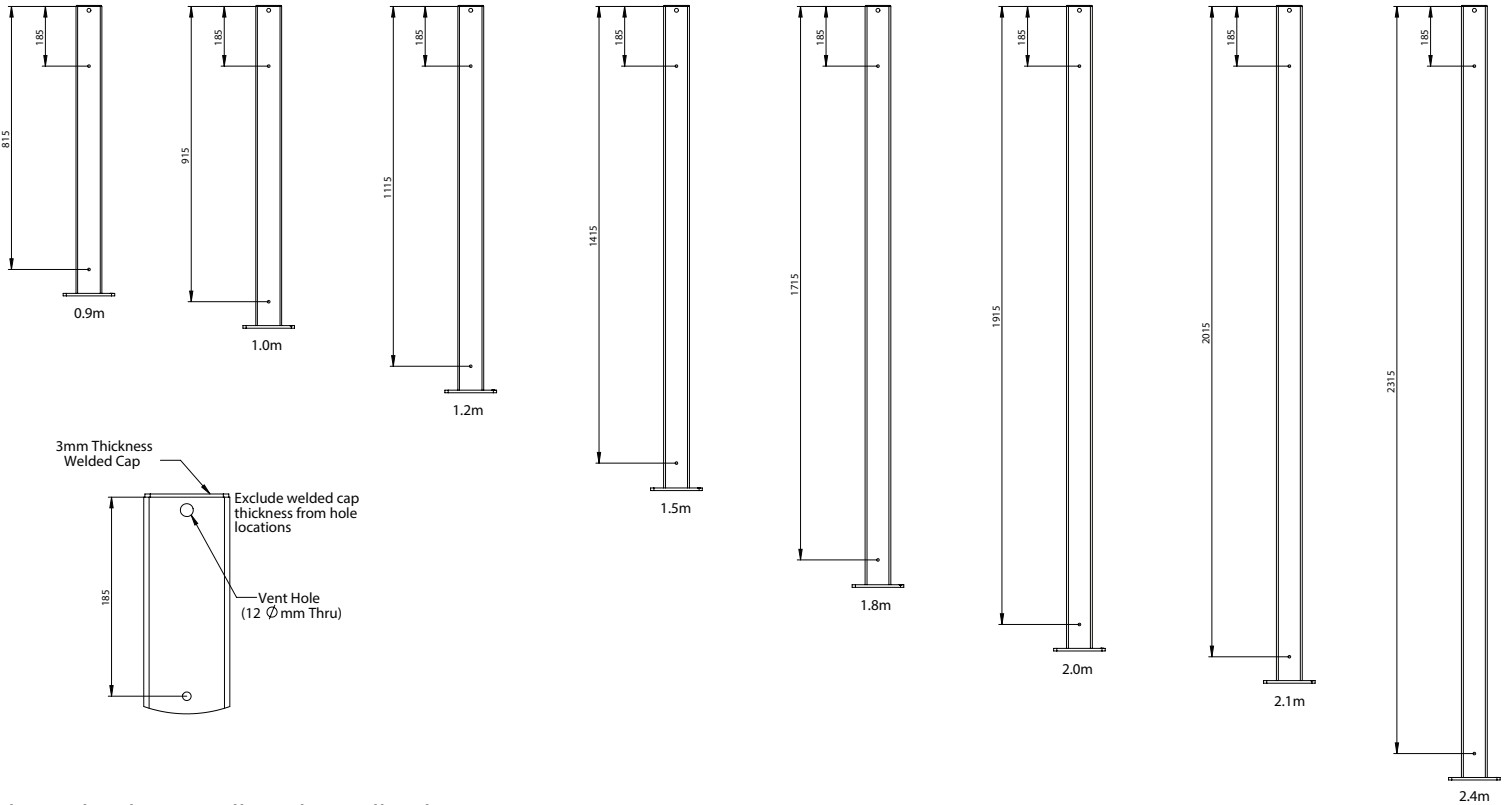
FlexiRail Railing Install Guide - Drill Hole Locations Bolt Down Posts - 0.9m to 2.4m High Systems
