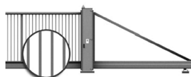
Closed box section infill 25x25 [mm], CARO arrangement, welded to the structure.
