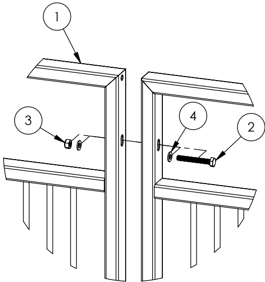
EXPLODED VIEW
