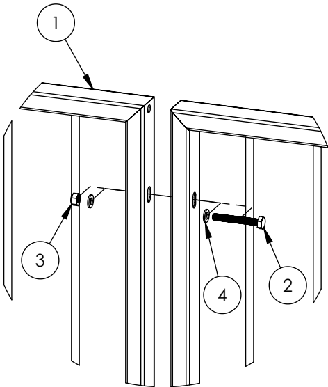
EXPLODED VIEW
