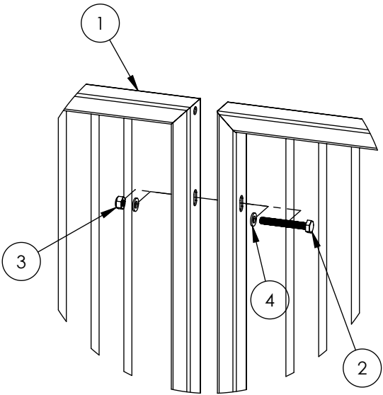
EXPLODED VIEW
