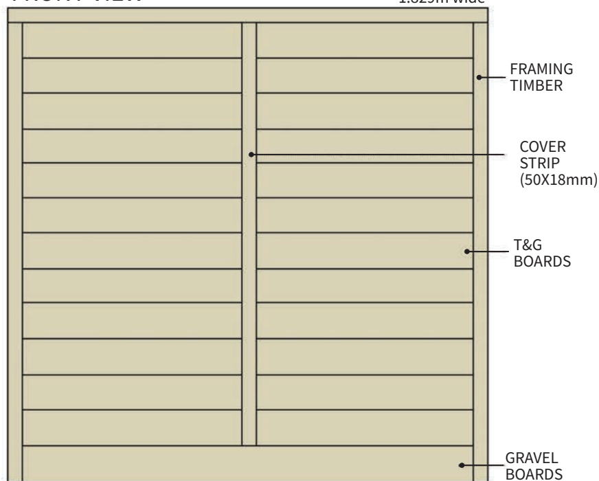
Gravel Board
