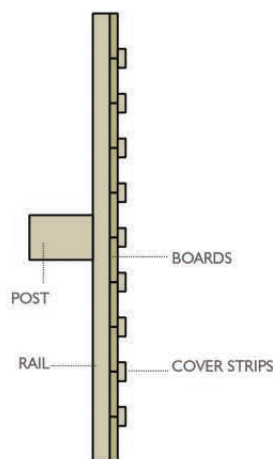
PLAN VIEW (Capping omitted)
