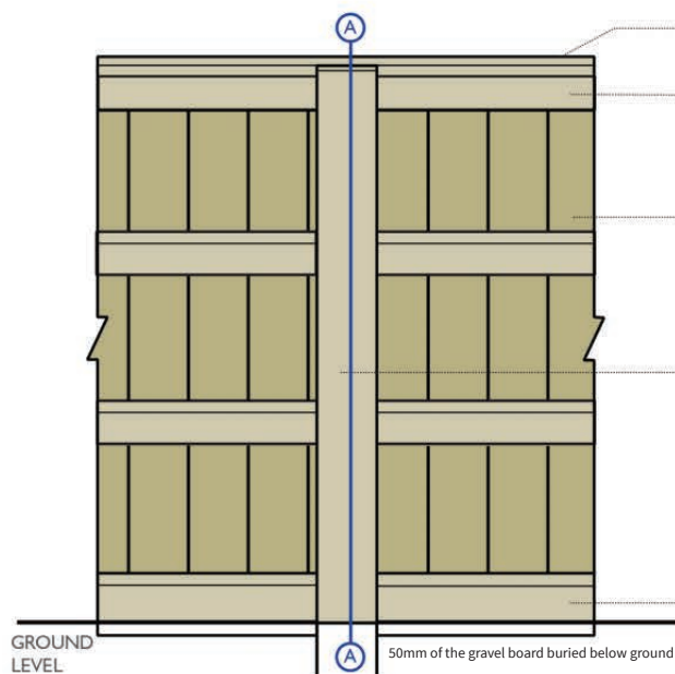
REAR VIEW
