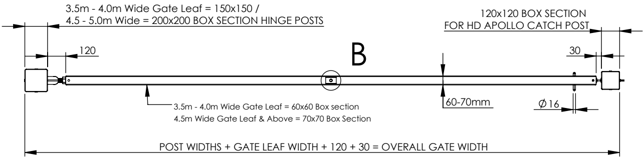
DETAIL B
