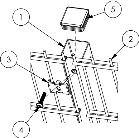
Exploded View
