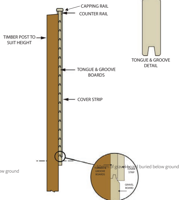
SIDE VIEW TIMBER POST
