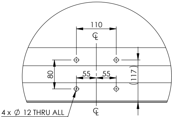
Hole Detail
