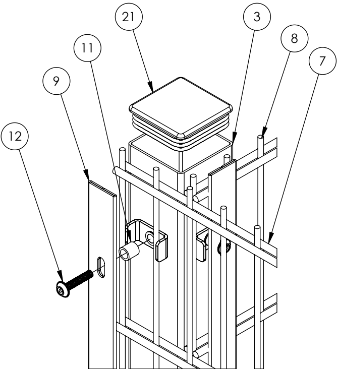
EXPLOADED VIEW
