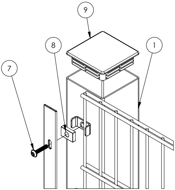
EXPLOADED VIEW
