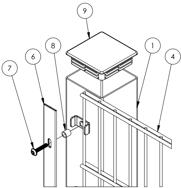
EXPLODED VIEW
