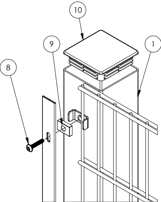
EXPLODED VIEW
