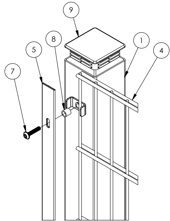
EXPLODED VIEW
