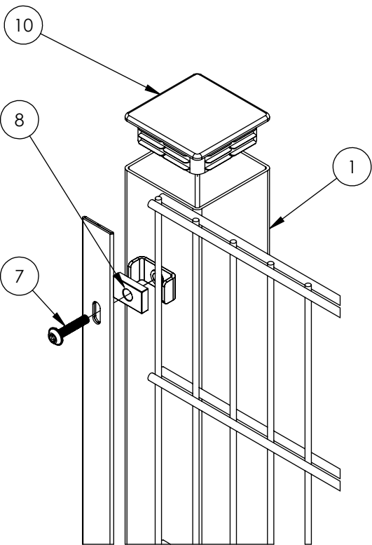
EXPLODED VIEW
