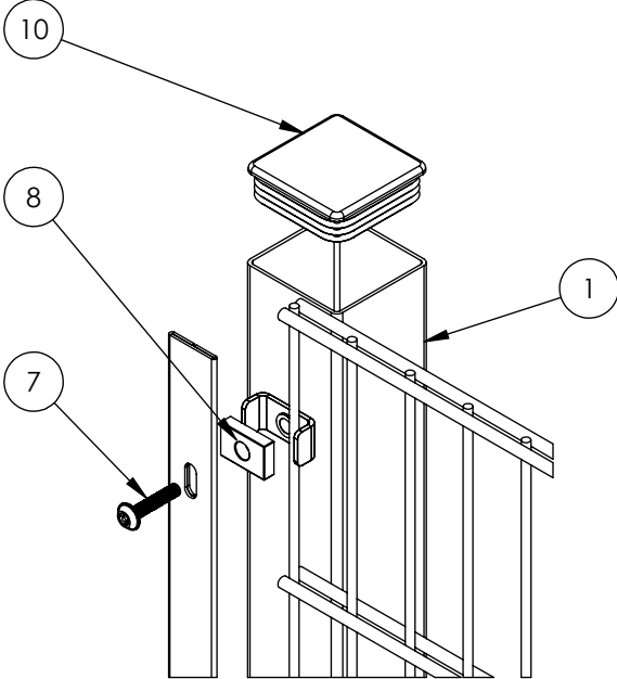
EXPLODED VIEW
