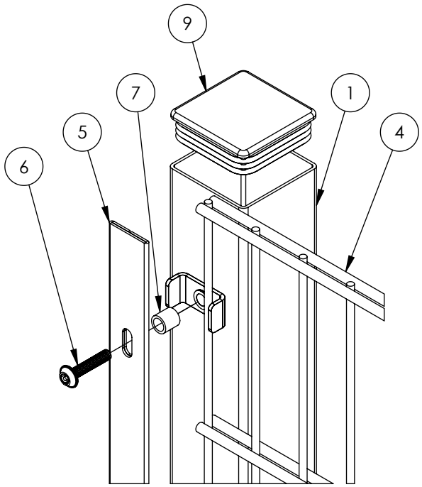
EXPLODED VIEW
