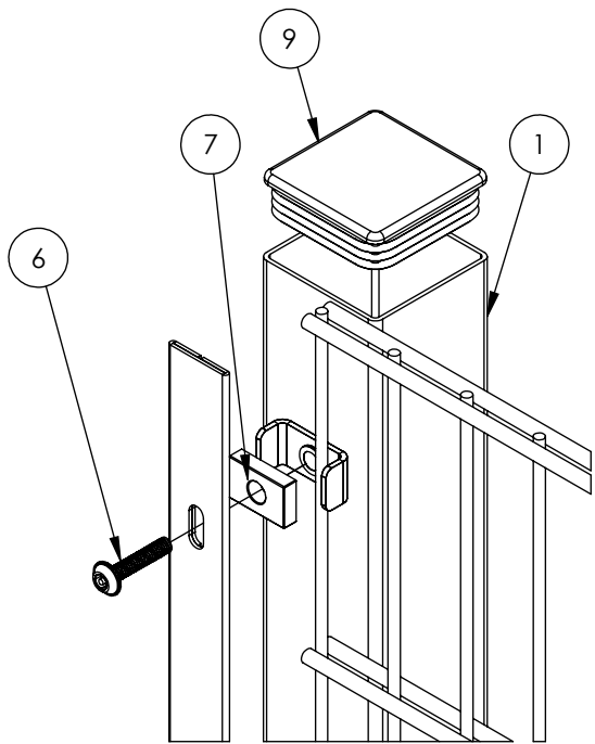
EXPLODED VIEW
