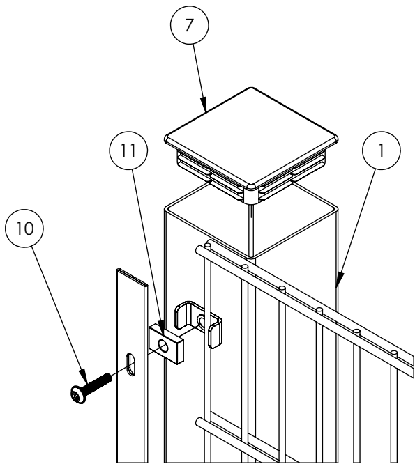
EXPLODED VIEW
