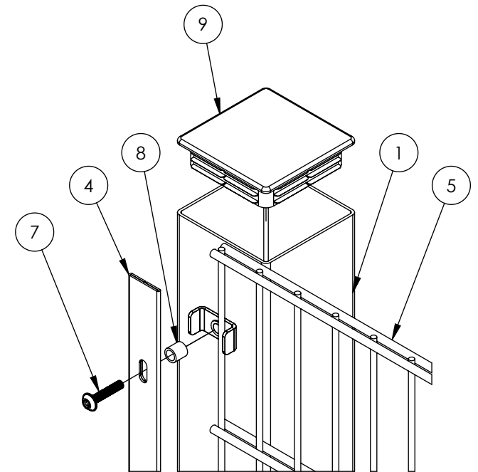
EXPLODED VIEW
