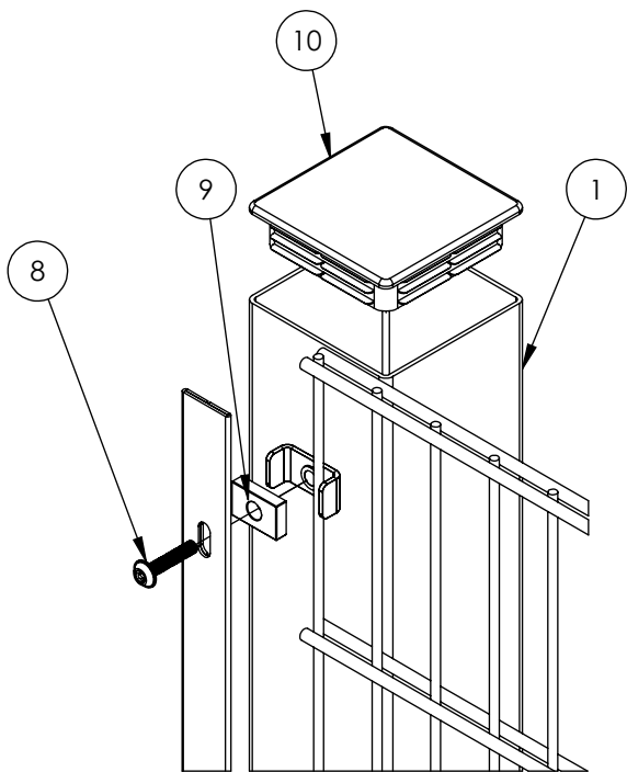
EXPLODED VIEW
