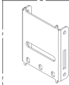
PART B ACCS-GATE-1110 Blank Single Slider Plate
