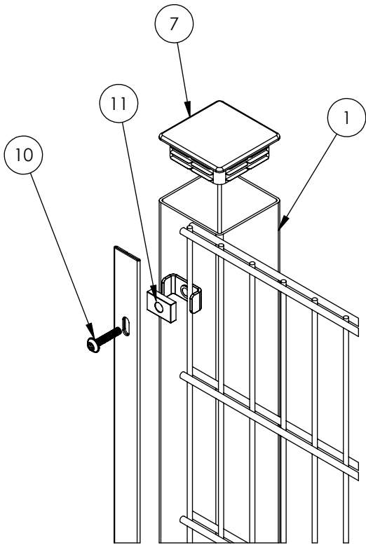
EXPLOADED VIEW
