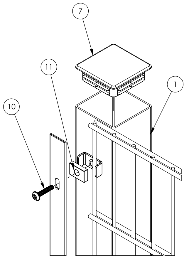
EXPLODED VIEW
