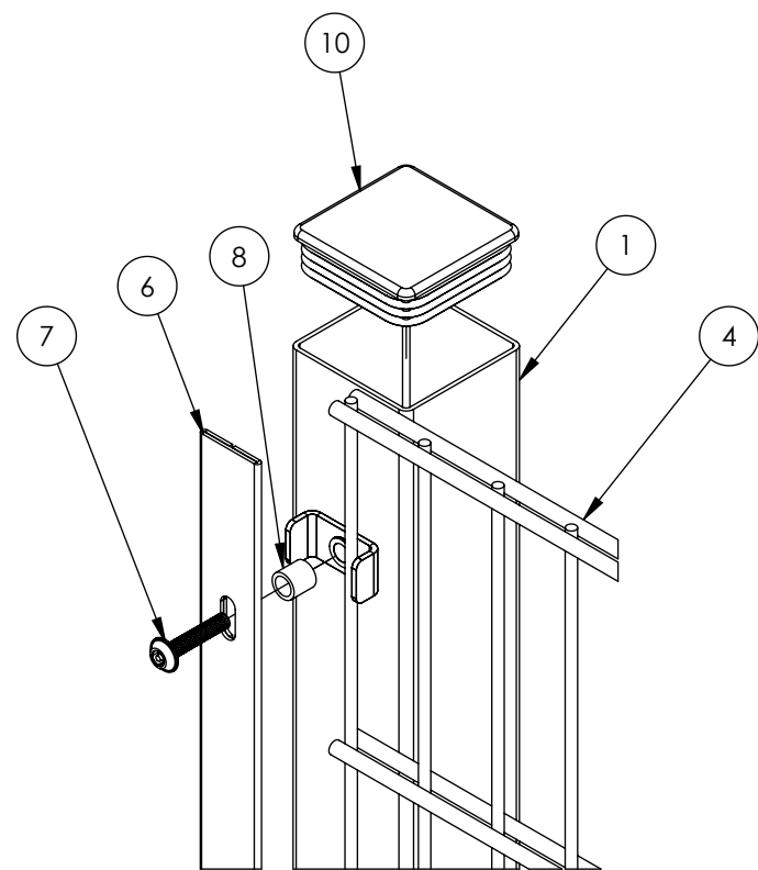
EXPLODED VIEW
