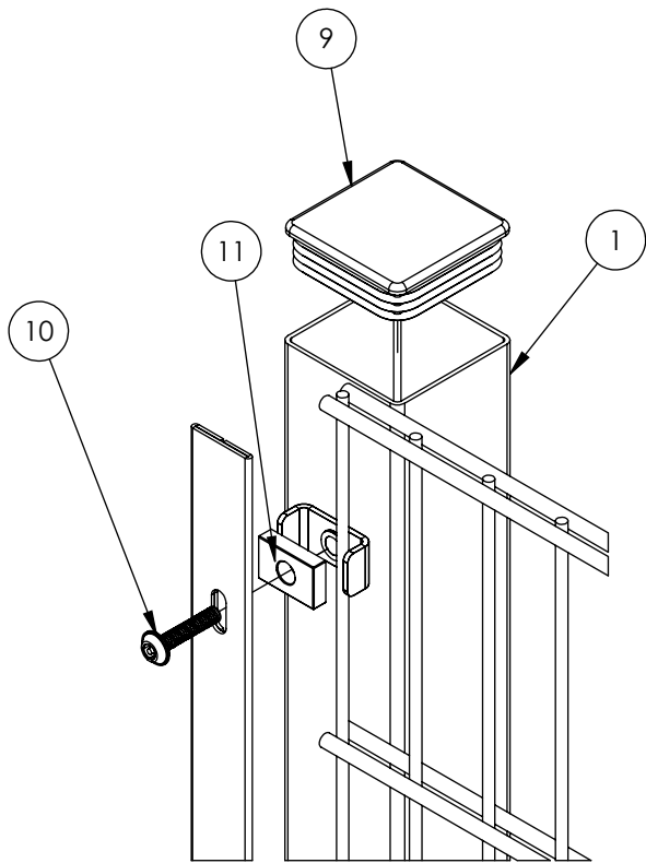
EXPLODED VIEW
