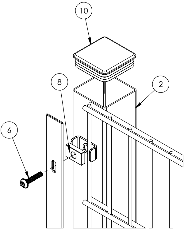
EXPLODED VIEW
