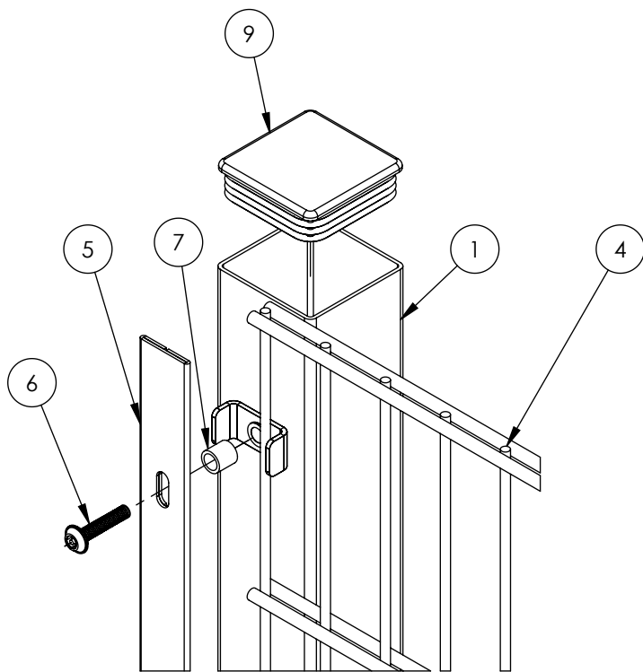
EXPLODED VIEW
