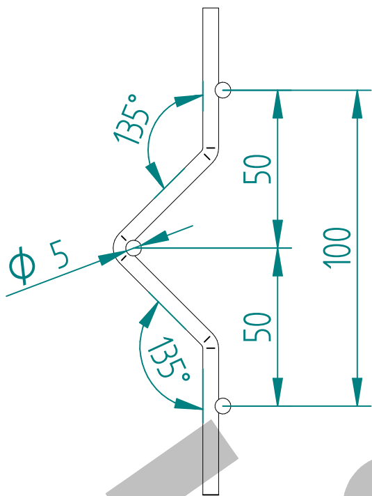
DETAIL C
