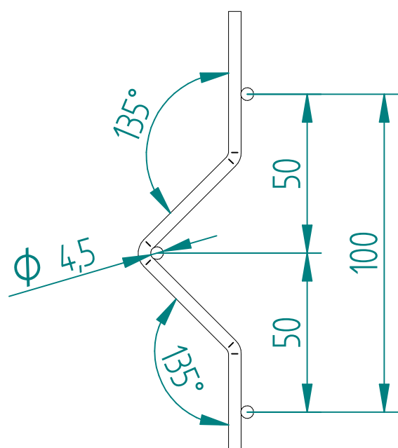
DETAIL C
