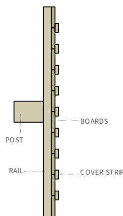
PLAN VIEW (Capping omitted)
