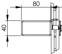
DETAIL C 3.0m Intermediate Post View
