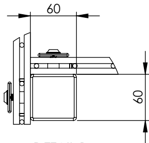
DETAIL B 1.2m Corner Post View
