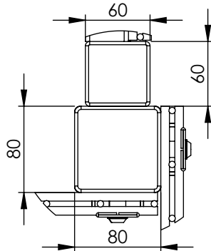
DETAIL D 3.0m Goal Post View
