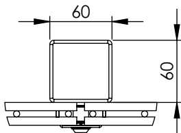
DETAIL A 1.2m Intermediate Post View
