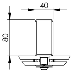
DETAIL A 3.0m Intermediate Post View
