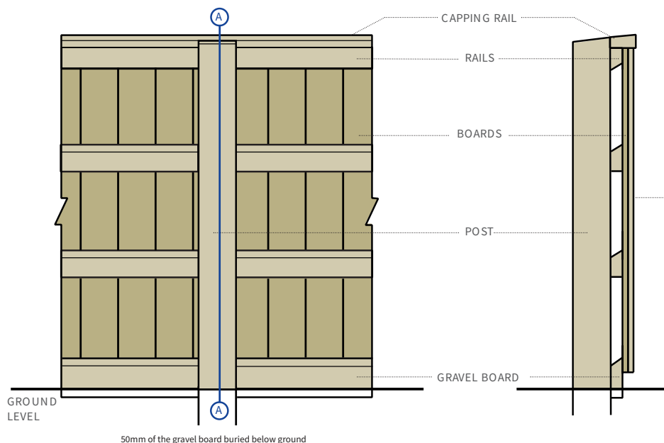
REAR VIEW
