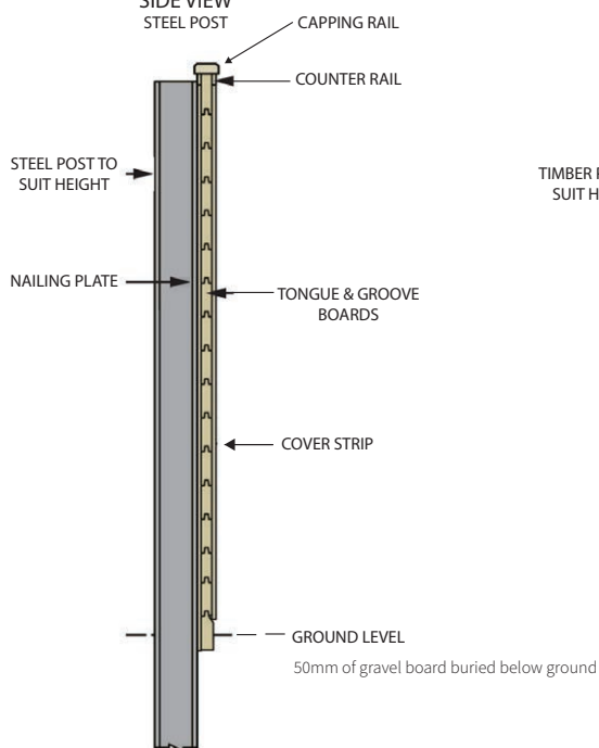
SIDE VIEW STEEL POST
