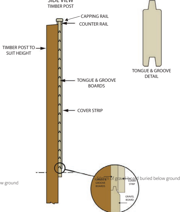
SIDE VIEW TIMBER POST
