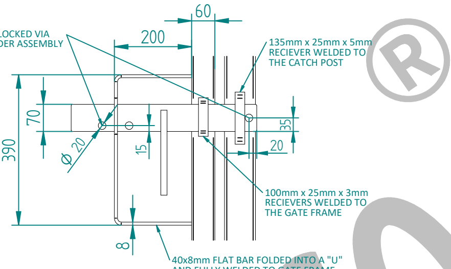
GENERIC SLIDER CONFIGURATION & LOCKING ARRANGEMENT
