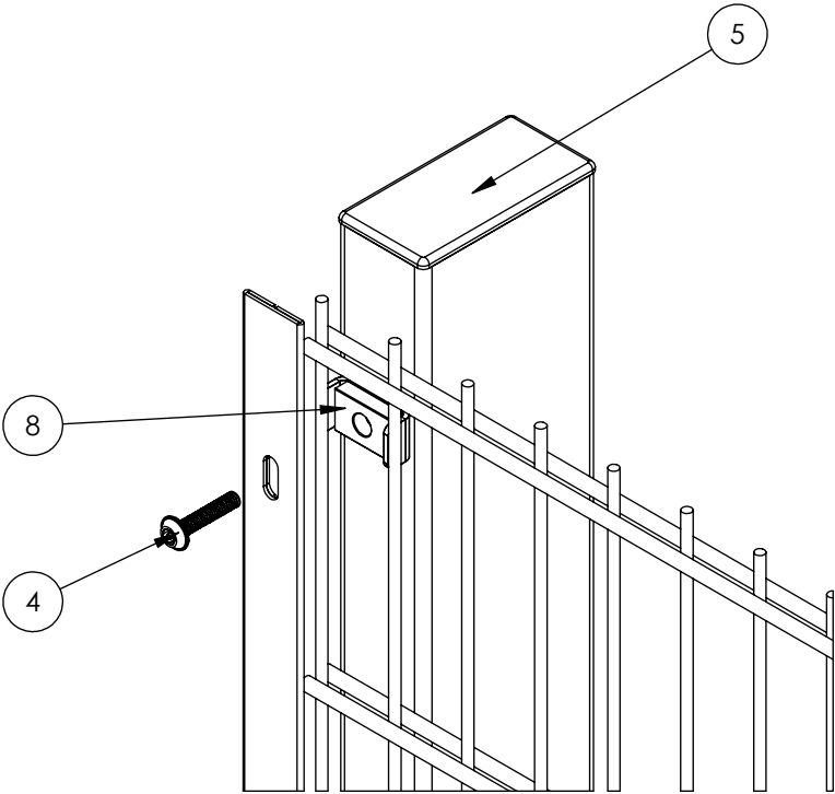
EXPLODED VIEW
