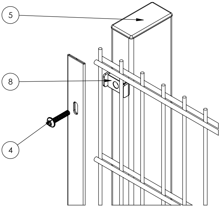
EXPLODED VIEW
