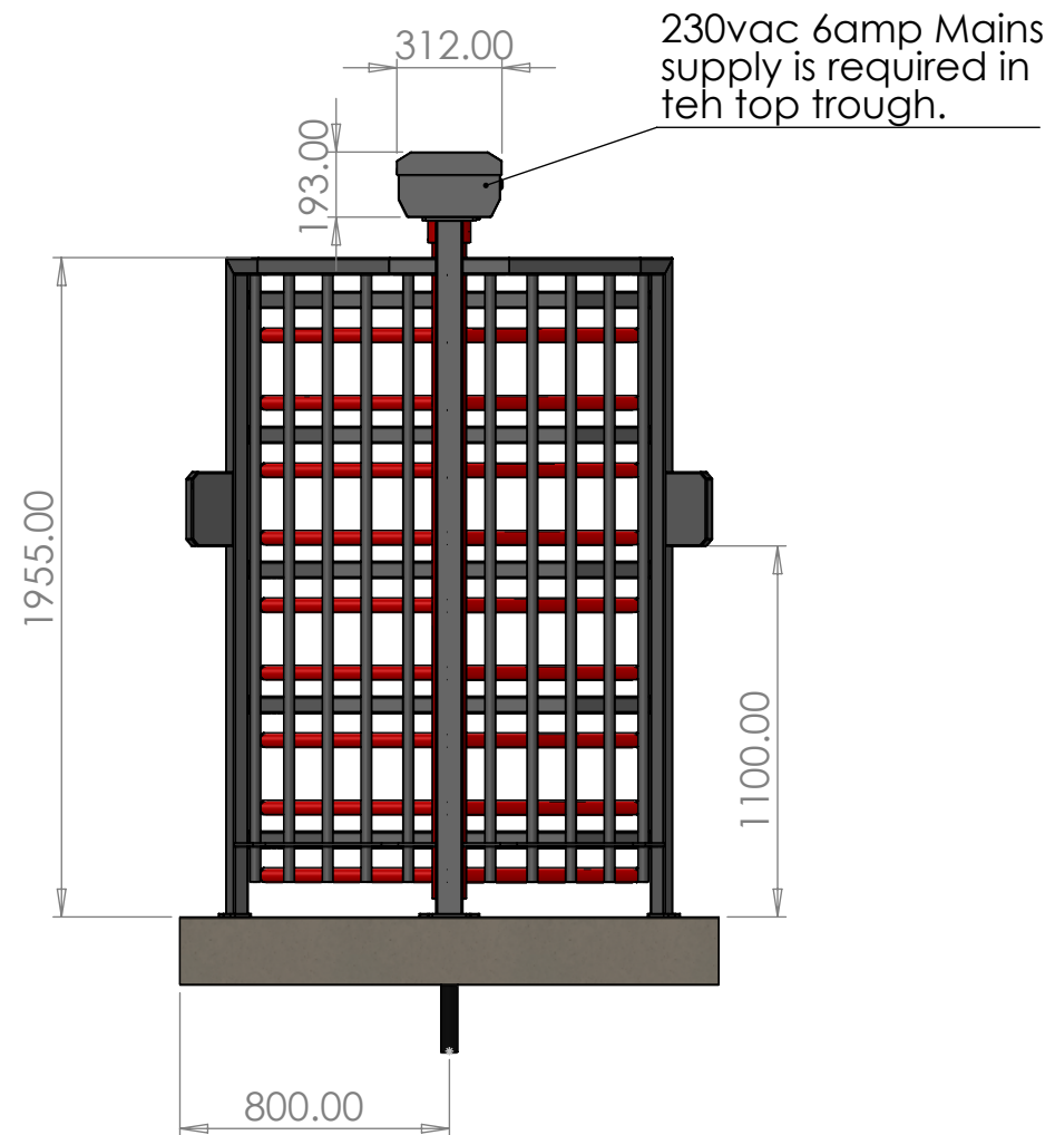
Access Control Facia Plate Dims
