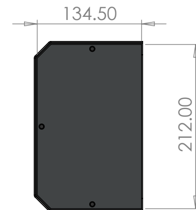
Access Control Facia Plate Dims
