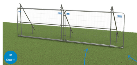
Back Braced (Scaffold Tube Frame) (Compliant with BS 5837:2012)
