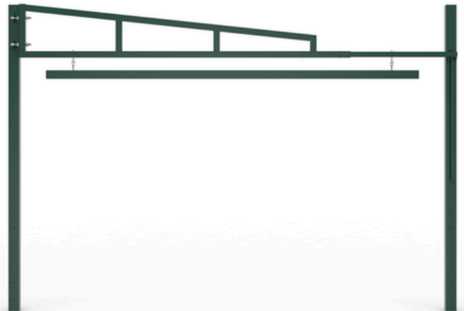
SWI-KIT-3060 - 2.2M High X 4.0M Wide Swing Barrier With Extended High Level Swing Arm Only Kit
